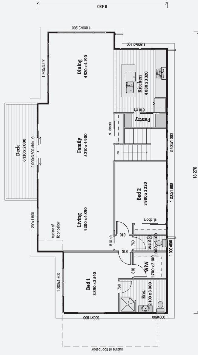
First Floor Area 141.4m 2 o/frame
