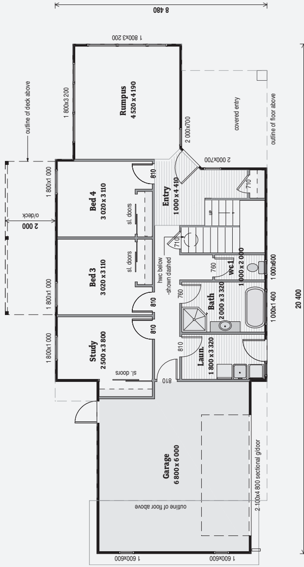
Ground Floor Area 137.5m 2 o/frame
